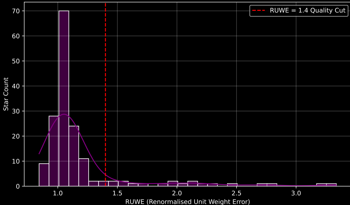
GAPOGEE DR17 Field [K2_C13_178-20_btx] RUWE Distribution (n= 165)
