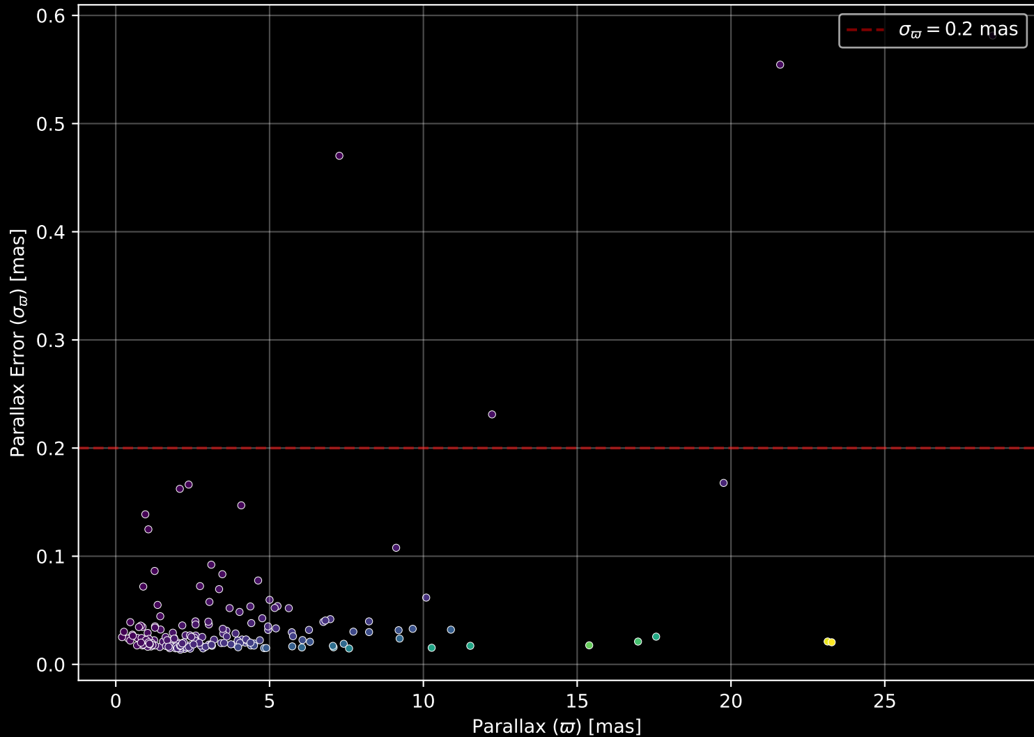
APOGEE DR17 Field: [K2_C13_178-20_btx] Parallax Quality (n= 172)
