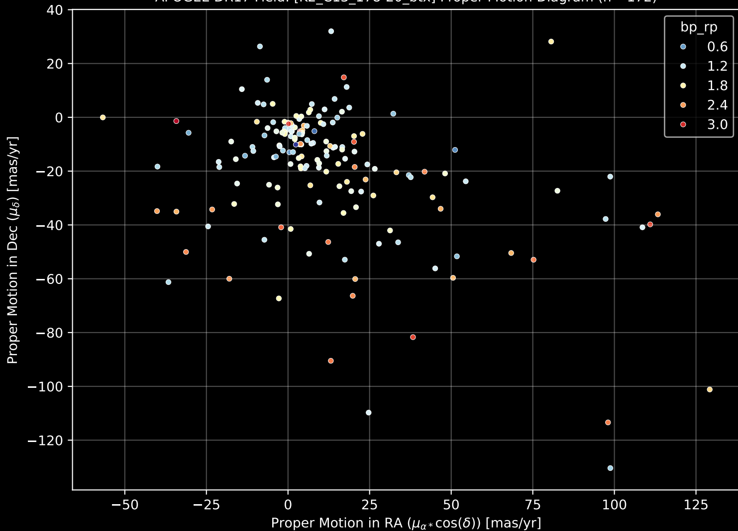
APOGEE DR17 Field: [K2_C13_178-20_btx] Proper Motion Diagram (n= 172)
