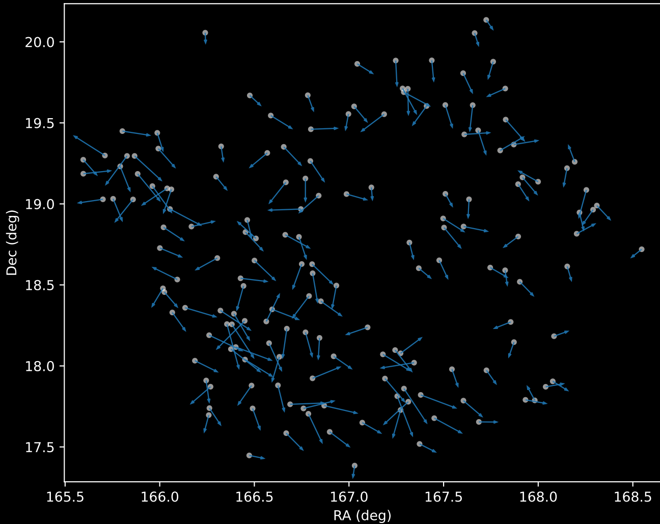
APOGEE DR17 Cluster 0 Proper Motion Vectors (n=161)
