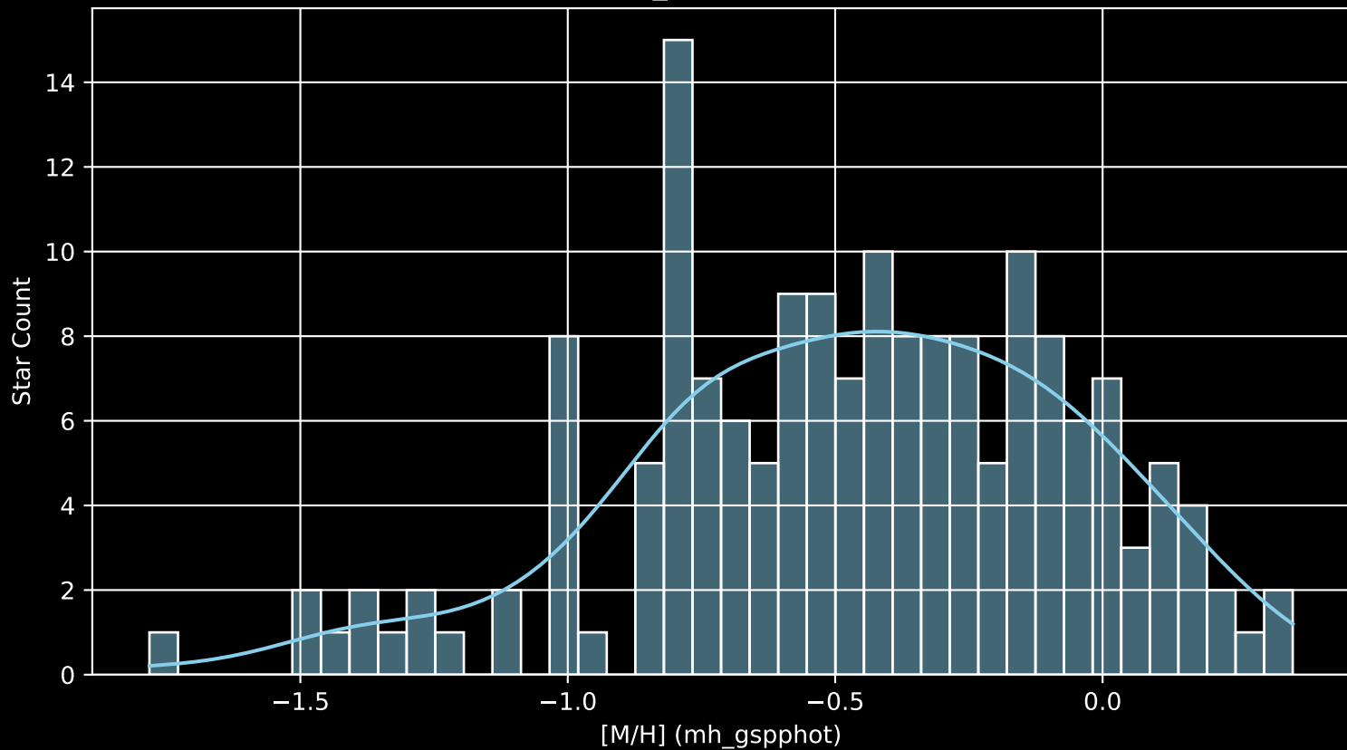
APOGEE DR17 Field: [K2_C13_178-20_btx [M/H] (mh_gspphot) (n= 171)
