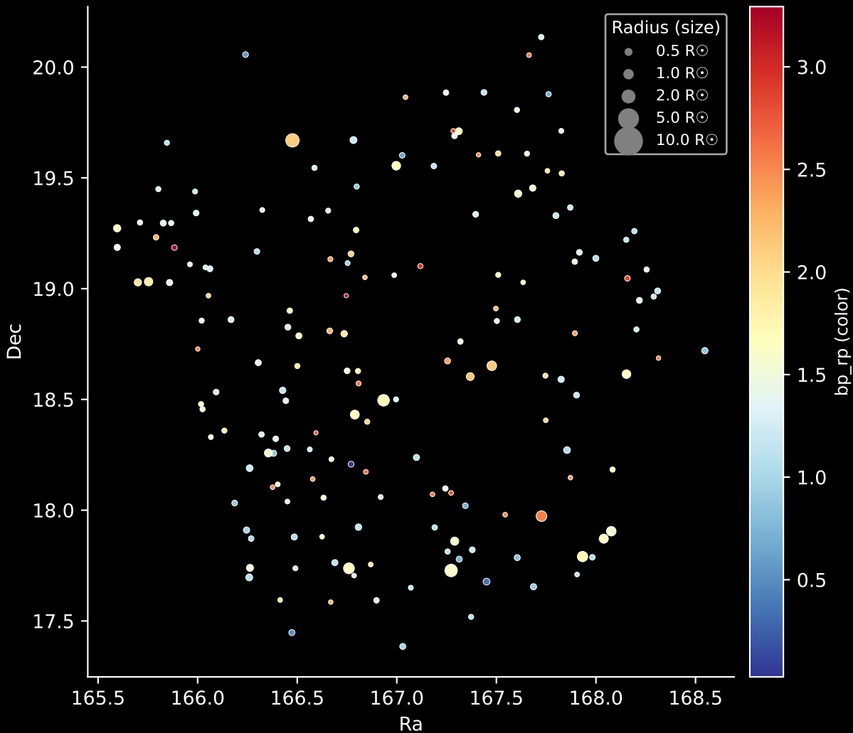
APOGEE DR17 Field: [K2_C13_178-20_btx] Stars: 172
