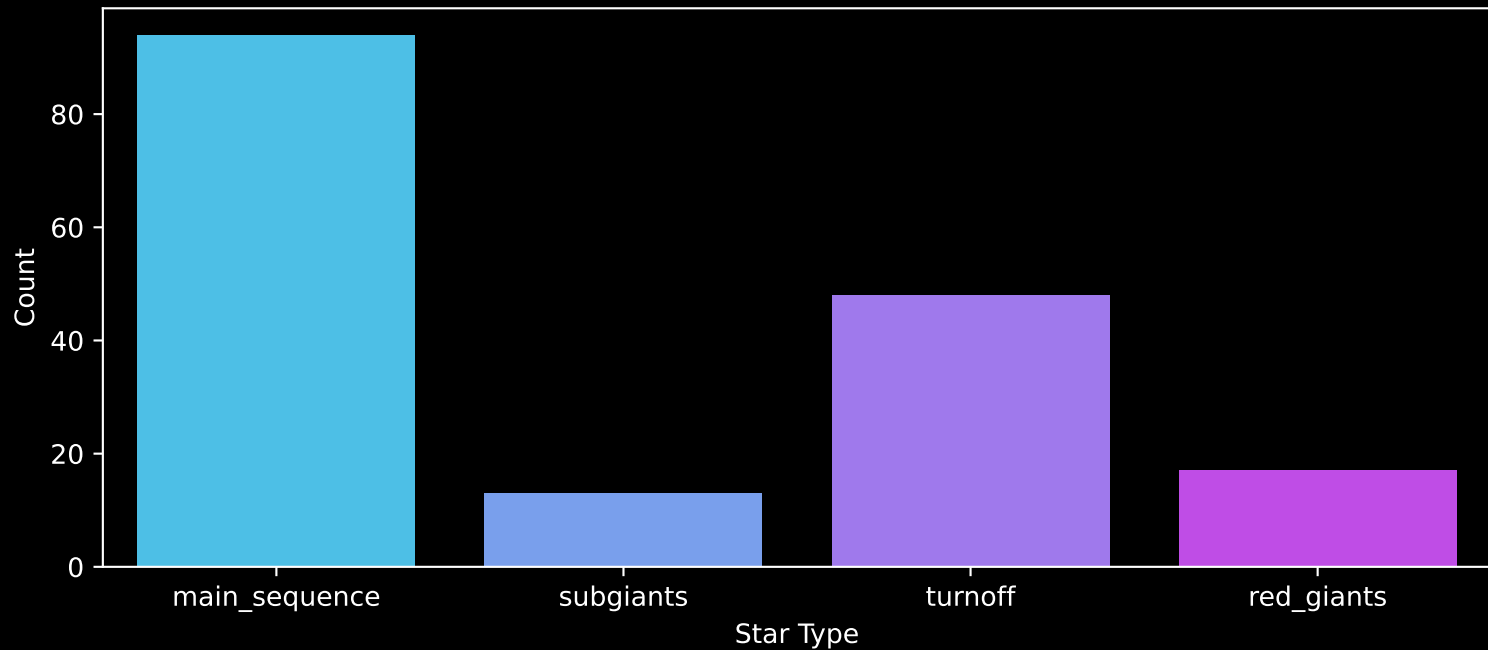
APOGEE DR17 Field: [K2_C13_178-20_btx] Count plot of Star Type
